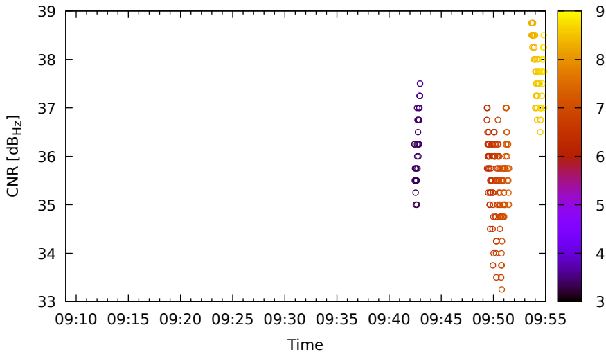
Timeline for R17 (G2) on LeicaGS18 - DOY 262
