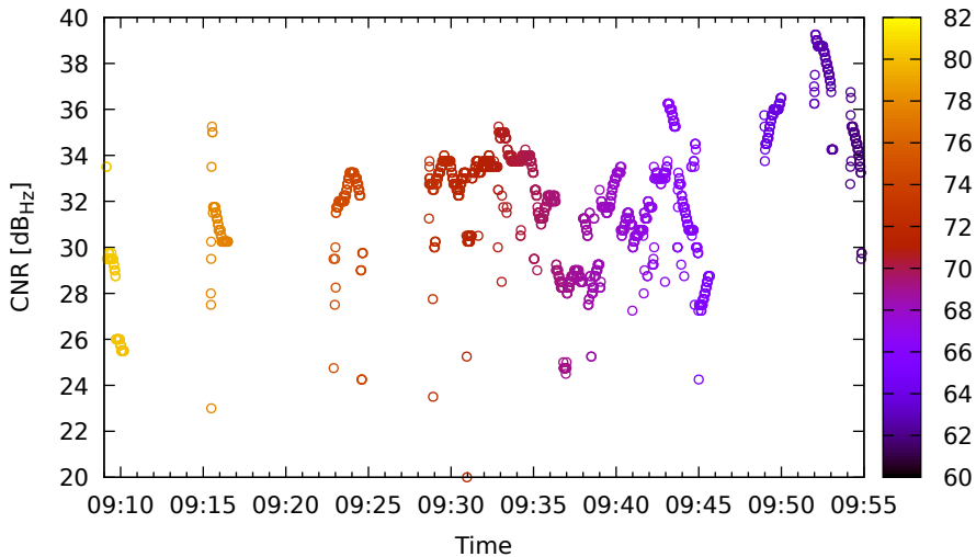
Timeline for C14 (B1) on Xiaomi11T - DOY 262
