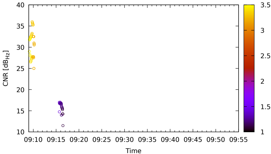
Timeline for C21 (B1) on Xiaomi11T - DOY 262
