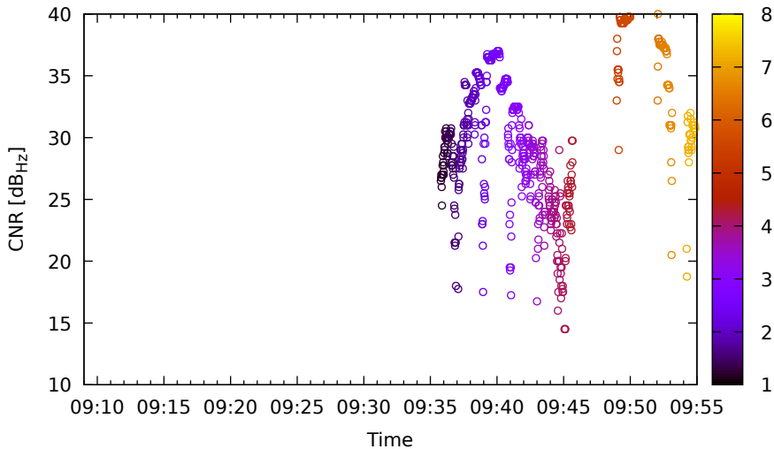
Timeline for E03 (E1) on Xiaomi11T - DOY 262
