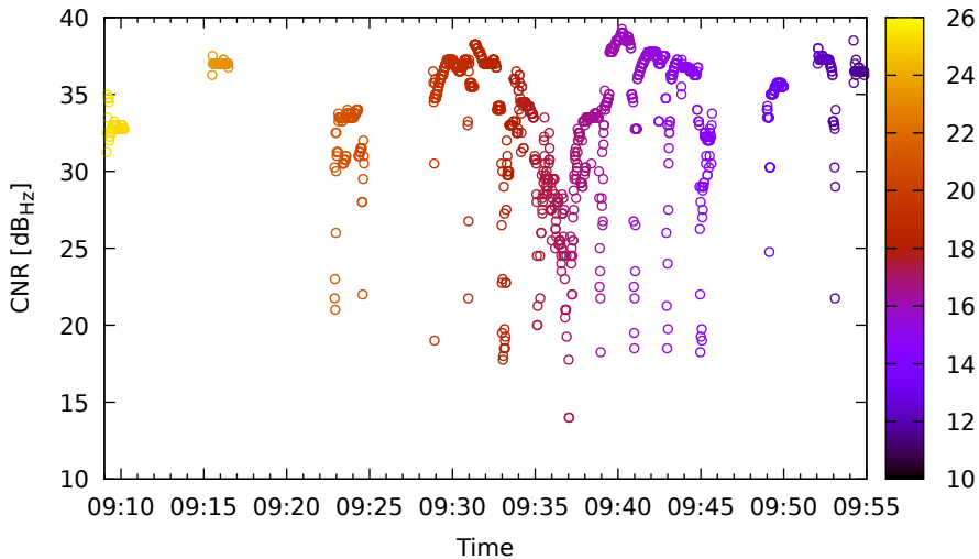
Timeline for E04 (E1) on Xiaomi11T - DOY 262
