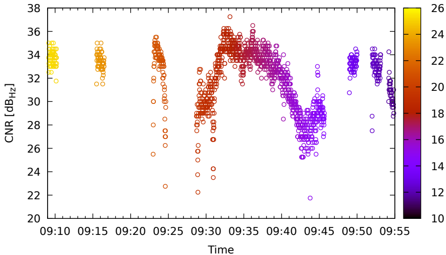
Timeline for E04 (E5a) on Xiaomi11T - DOY 262
