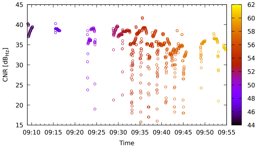
Timeline for E34 (E1) on Xiaomi11T - DOY 262
