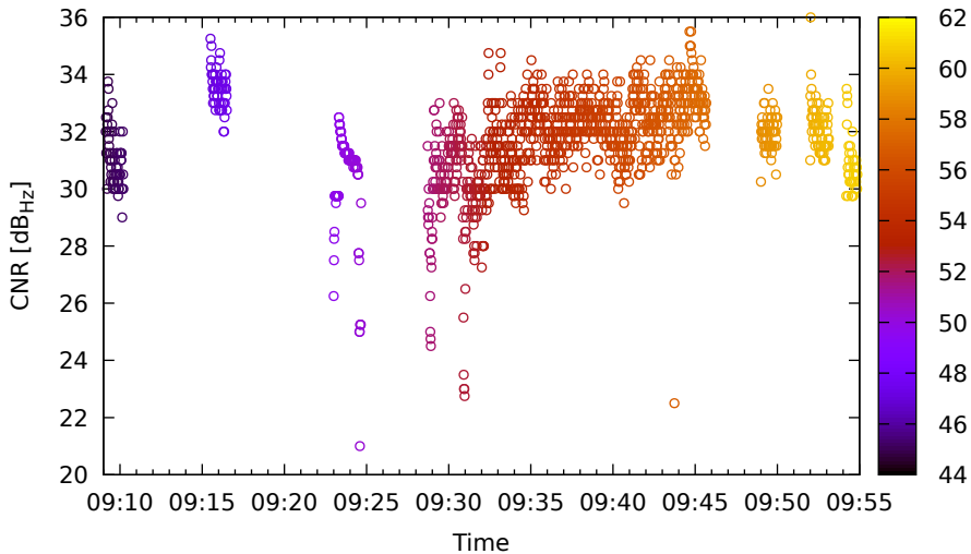
Timeline for E34 (E5a) on Xiaomi11T - DOY 262
