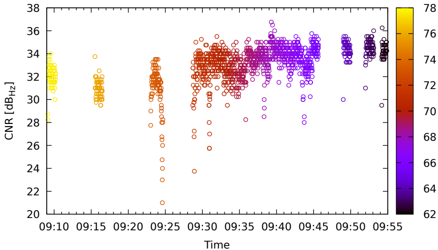
Timeline for E36 (E5a) on Xiaomi11T - DOY 262
