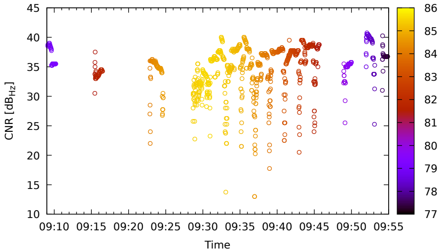
Timeline for G01 (L1) on Xiaomi11T - DOY 262
