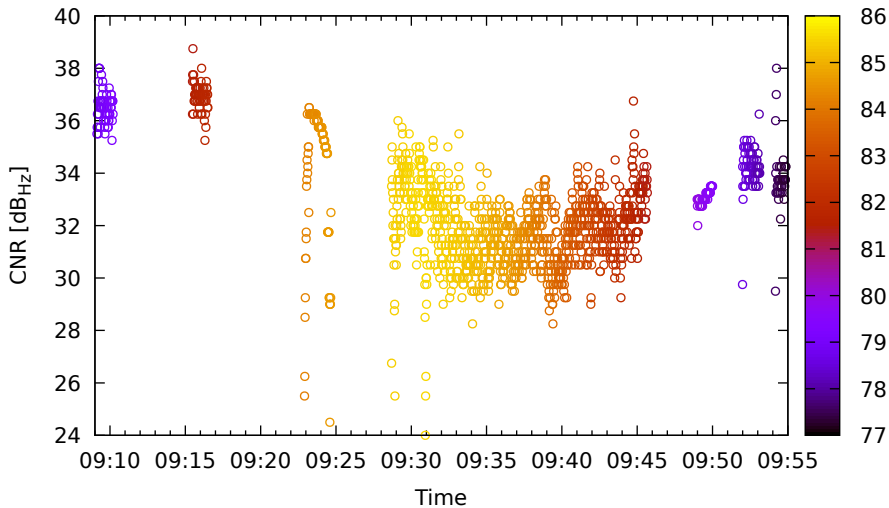
Timeline for G01 (L5) on Xiaomi11T - DOY 262
