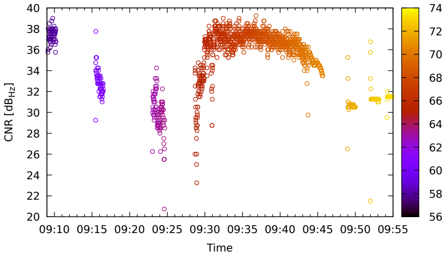
Timeline for G03 (L5) on Xiaomi11T - DOY 262
