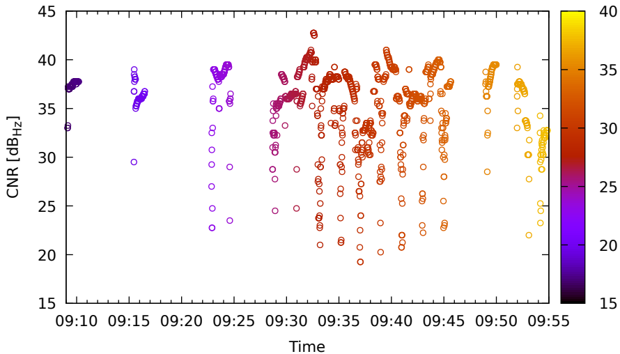
Timeline for G04 (L1) on Xiaomi11T - DOY 262
