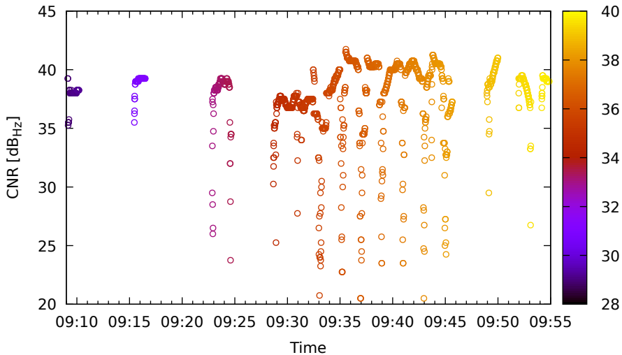
Timeline for G17 (L1) on Xiaomi11T - DOY 262
