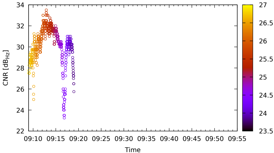
Timeline for E11 (E5a) on XiaomiMi8 - DOY 262
