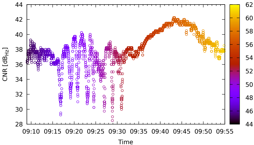
Timeline for E34 (E5a) on XiaomiMi8 - DOY 262
