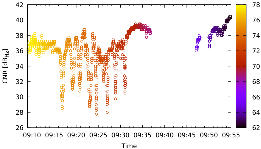
Timeline for E36 (E5a) on XiaomiMi8 - DOY 262
