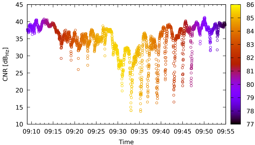
Timeline for G01 (L1) on XiaomiMi8 - DOY 262
