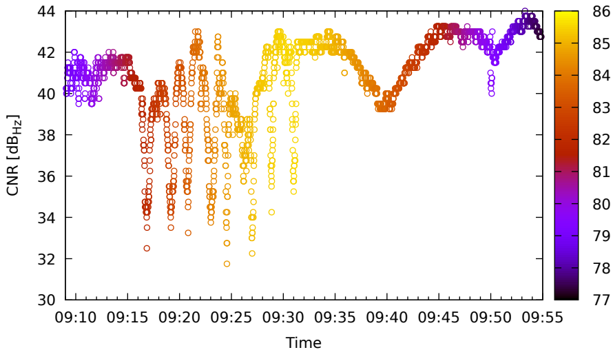
Timeline for G01 (L5) on XiaomiMi8 - DOY 262
