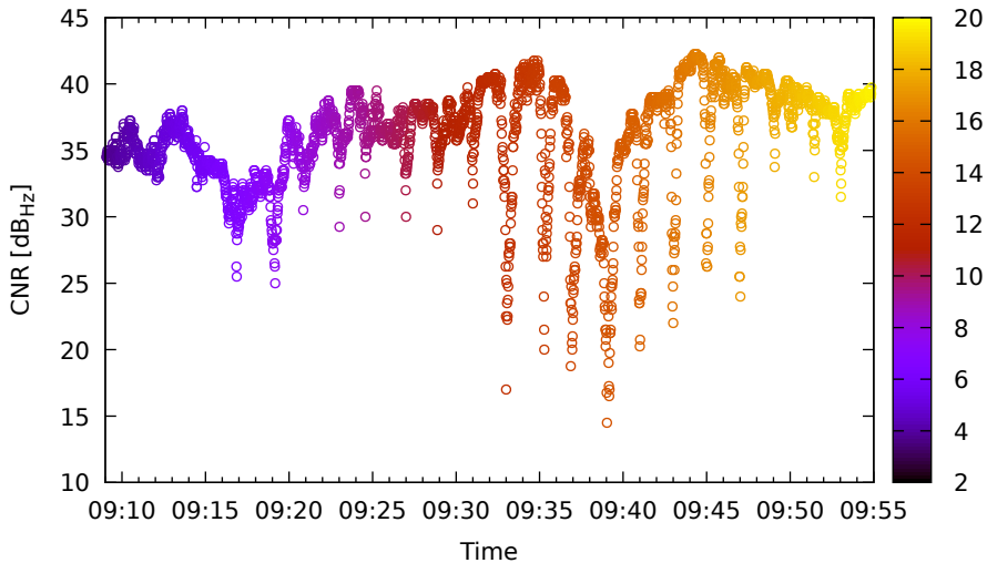
Timeline for G19 (L1) on XiaomiMi8 - DOY 262
