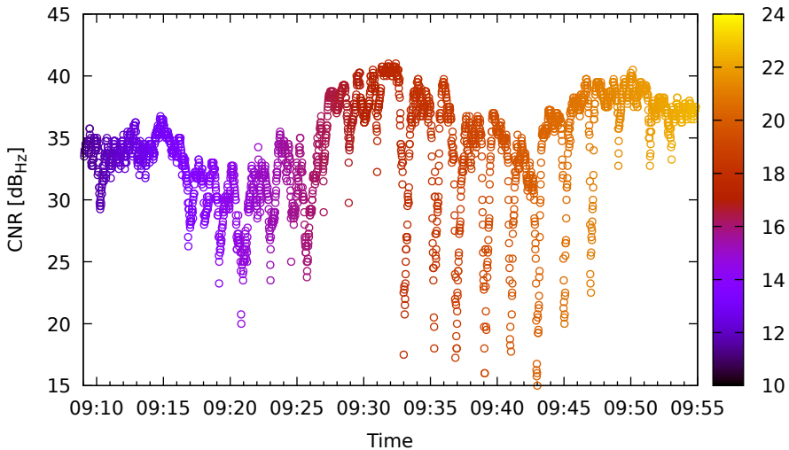
Timeline for G31 (L1) on XiaomiMi8 - DOY 262
