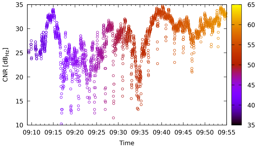
Timeline for R01 (G1) on XiaomiMi8 - DOY 262
