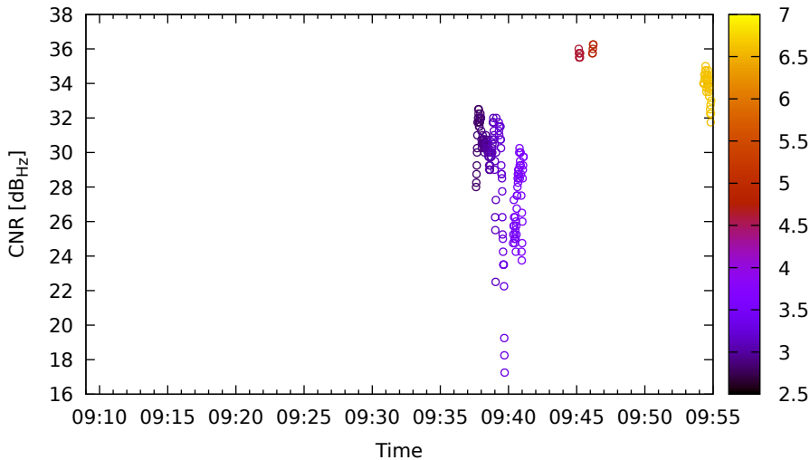
Timeline for R09 (G1) on XiaomiMi8 - DOY 262
