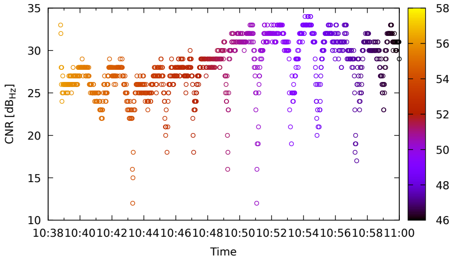
Timeline for G01 (G1) on HuaweiP40 - DOY 262
