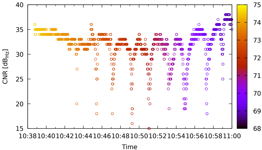
Timeline for G03 (G1) on HuaweiP40 - DOY 262
