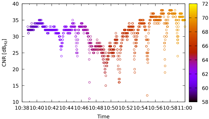
Timeline for G04 (G1) on HuaweiP40 - DOY 262
