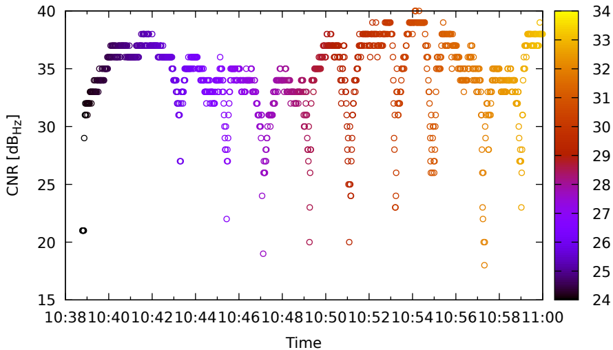
Timeline for G09 (L1) on HuaweiP40 - DOY 262
