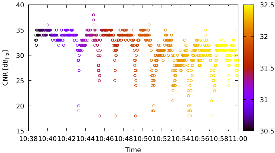
Timeline for G19 (G1) on HuaweiP40 - DOY 262
