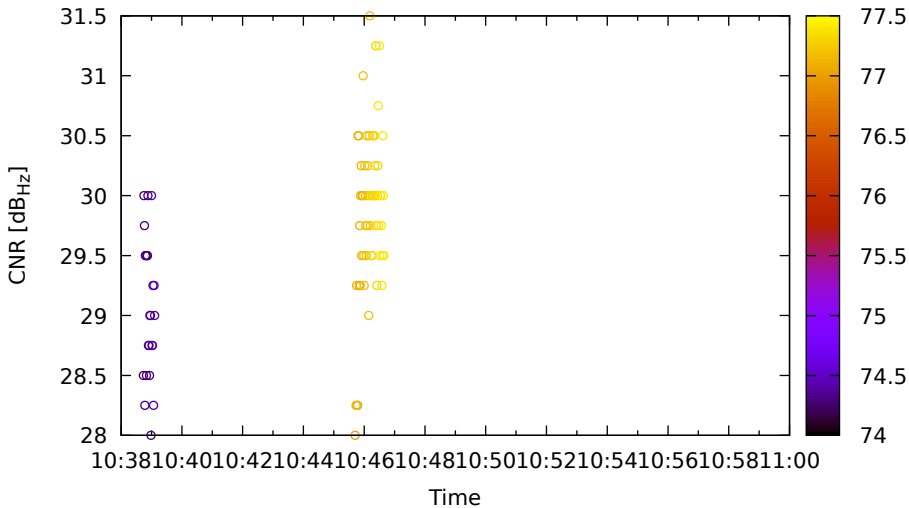
Timeline for E05 (E5a) on Xiaomi11T - DOY 262
