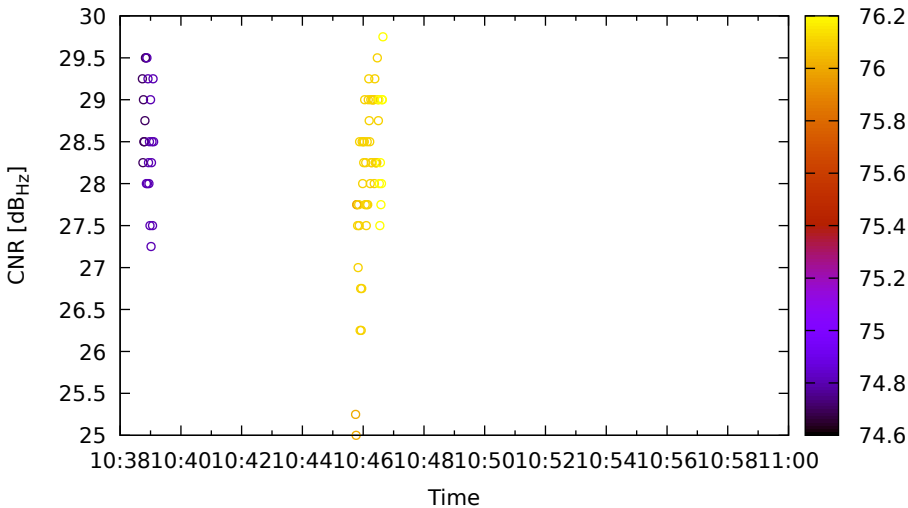
Timeline for E34 (E5a) on Xiaomi11T - DOY 262
