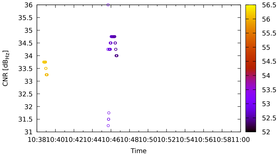
Timeline for G01 (L1) on Xiaomi11T - DOY 262
