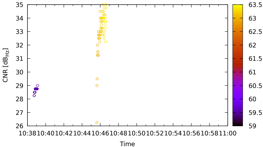
Timeline for G04 (L5) on Xiaomi11T - DOY 262
