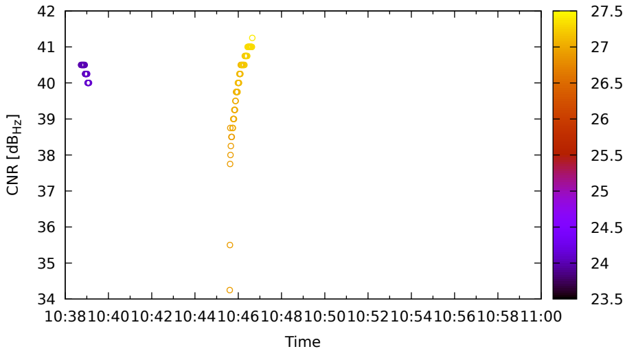
Timeline for G09 (L1) on Xiaomi11T - DOY 262
