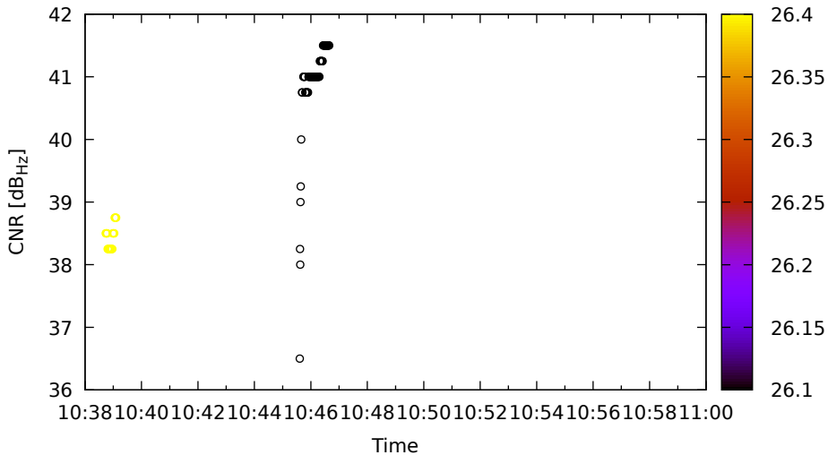
Timeline for G31 (L1) on Xiaomi11T - DOY 262
