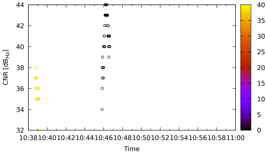
Timeline for R08 (G1) on Xiaomi11T - DOY 262
