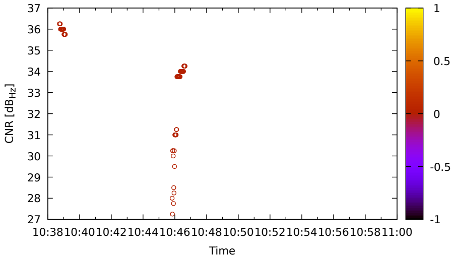
Timeline for R10 (G1) on Xiaomi11T - DOY 262
