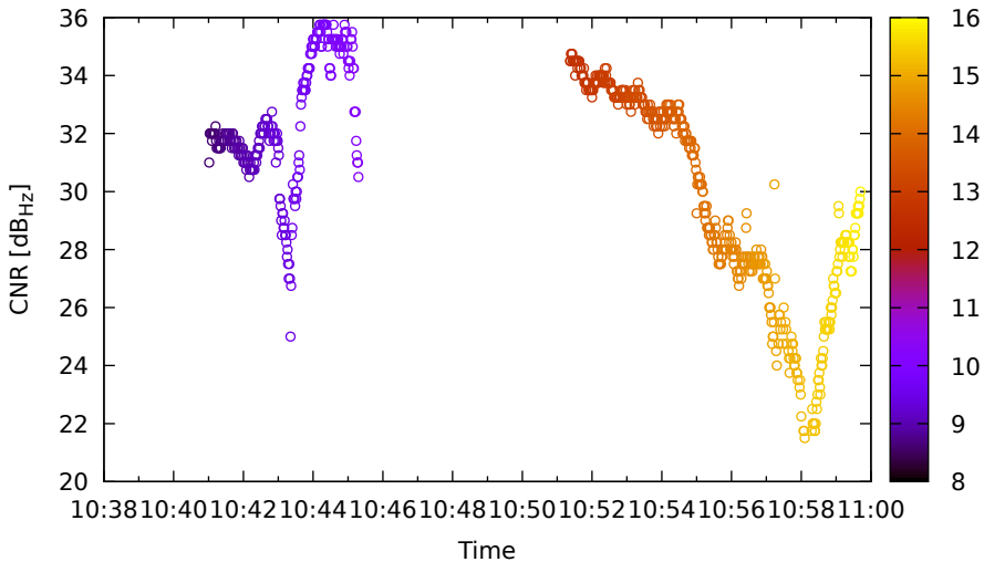
Timeline for G06 (L5) on XiaomiMi8 - DOY 262
