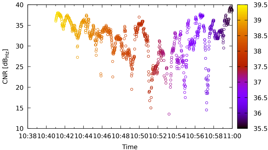
Timeline for G17 (L1) on XiaomiMi8 - DOY 262
