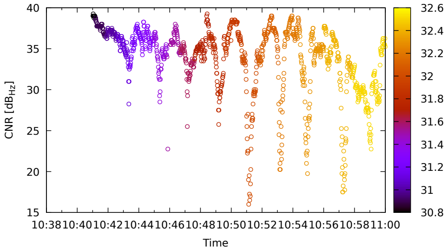
Timeline for G19 (L1) on XiaomiMi8 - DOY 262
