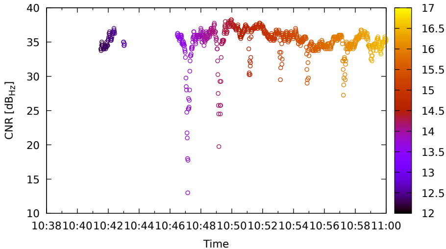
Timeline for R10 (G1) on XiaomiMi8 - DOY 262
