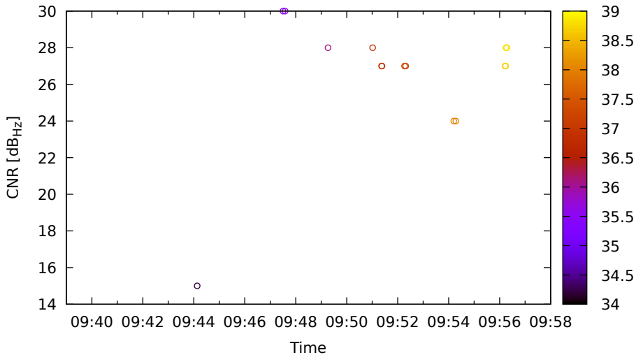
Timeline for E04 (E5a) on HuaweiP40 - DOY 263
