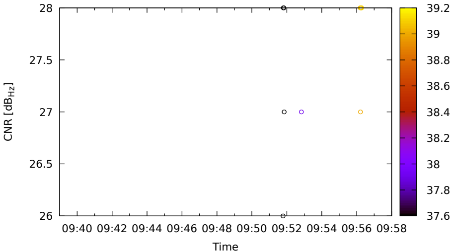
Timeline for E11 (E5a) on HuaweiP40 - DOY 263
