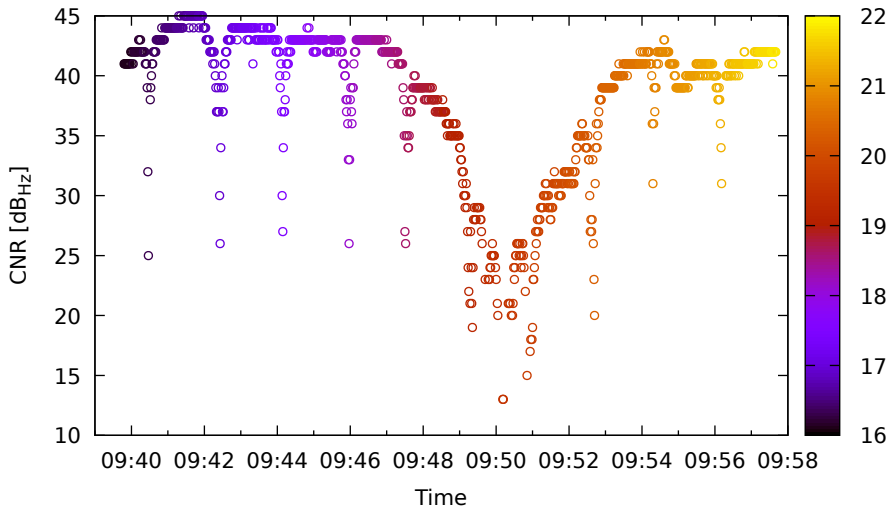
Timeline for G19 (L1) on HuaweiP40 - DOY 263
