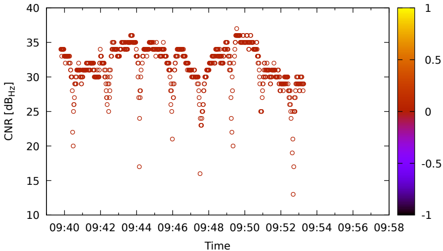
Timeline for G28 (L1) on HuaweiP40 - DOY 263
