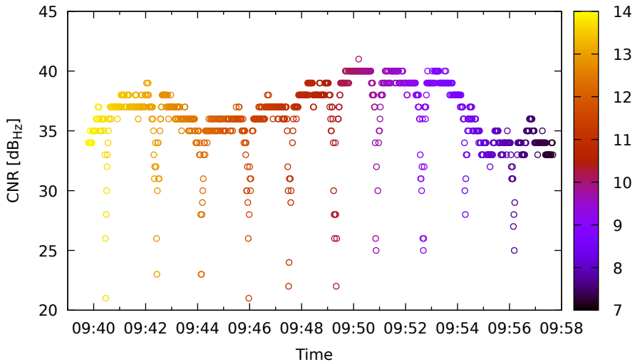
Timeline for G32 (L1) on HuaweiP40 - DOY 263
