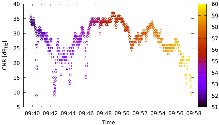
Timeline for R02 (G1) on HuaweiP40 - DOY 263
