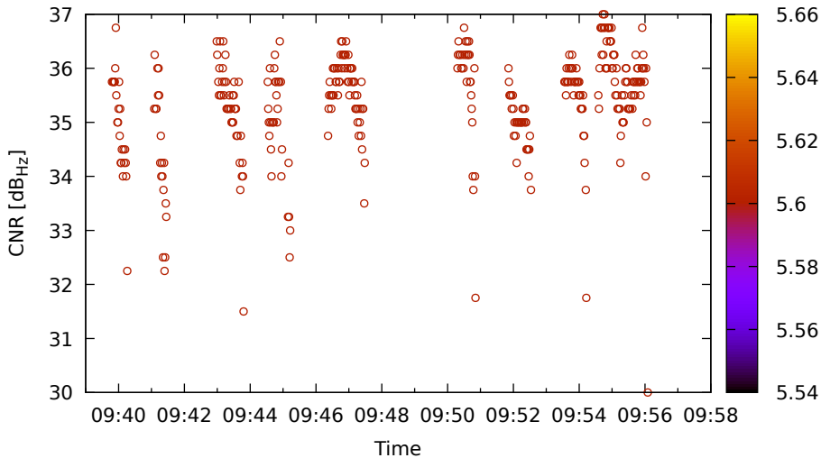
Timeline for C02 (B1) on LeicaGS18 - DOY 263
