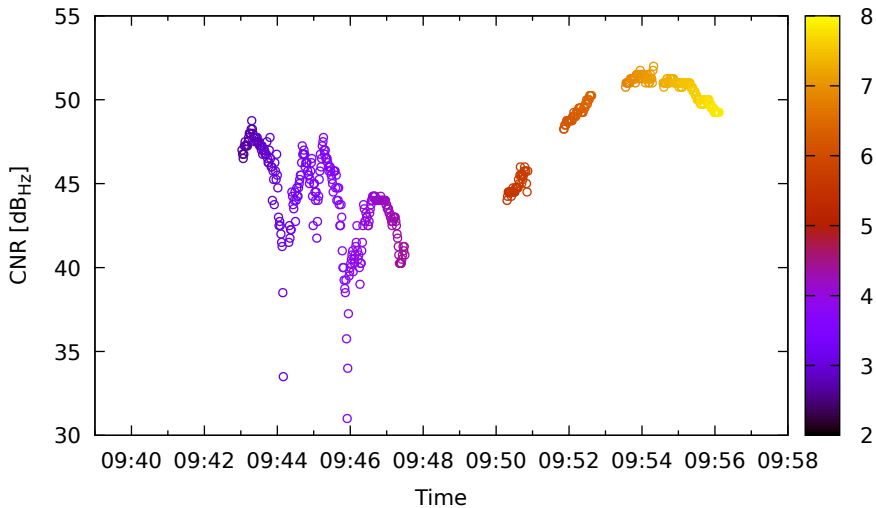
Timeline for G09 (L5) on LeicaGS18 - DOY 263
