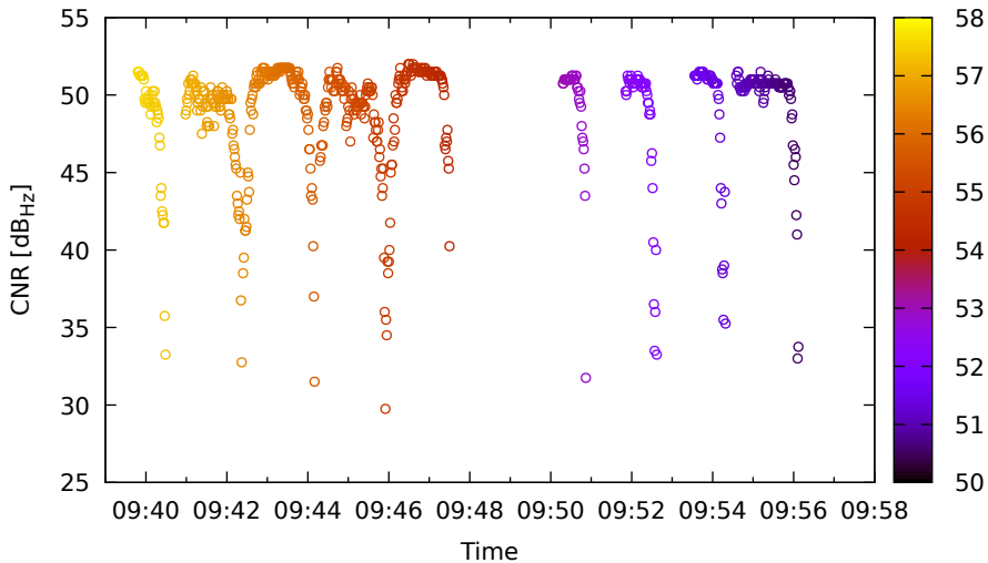
Timeline for G21 (L1) on LeicaGS18 - DOY 263
