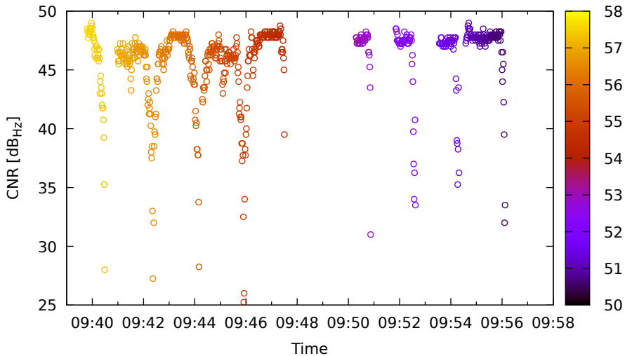
Timeline for G21 (L2) on LeicaGS18 - DOY 263
